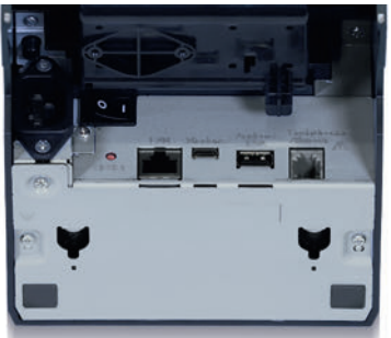
TSP100IV Multi-Connectivity Interfaces
